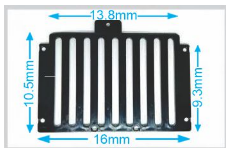
LS/F-049 REJILLA 9 COLORES NEEDLE BAR # FX0613020900®
