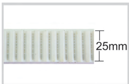
LS/C-360S BANDA PASO AT5, ANCHO 25MM
